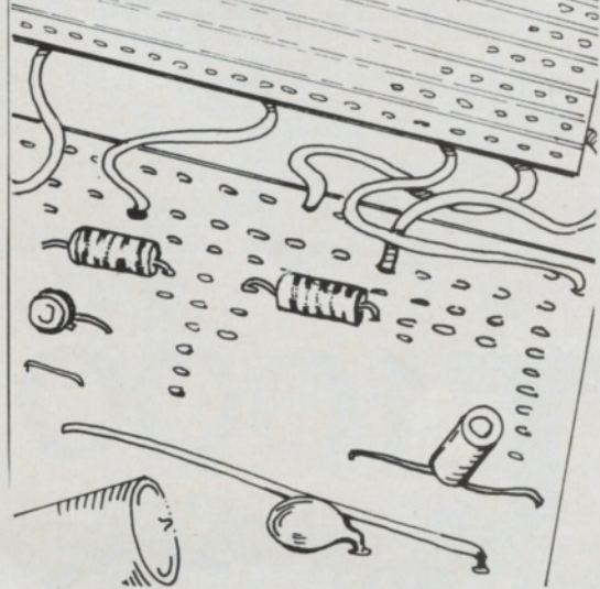
Figure 16: Connect small board to edge connector
